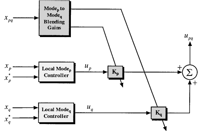
Fig. 2 Mode transition controller structure.
