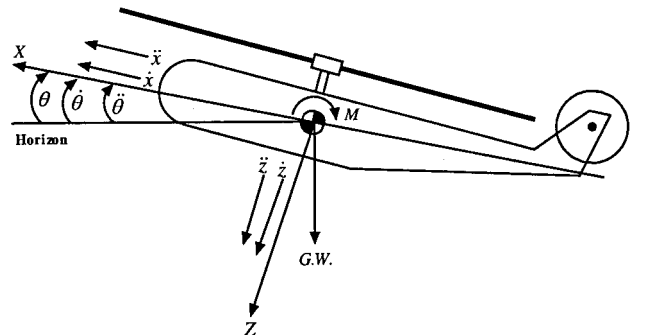
Fig. 4 Side view of helicopter's axis system.
