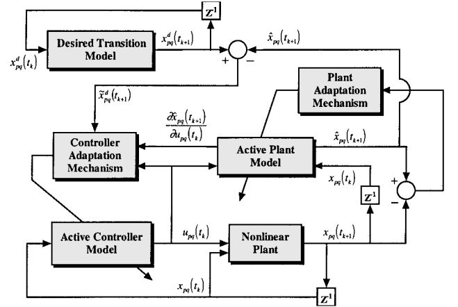
Fig. 3 Configuration for indirect adaptive mode transition control.
